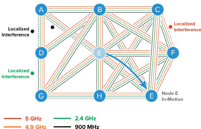
Diagram showing how a Rajant network with LX5 BreadCrums adapts to changes caused by the movement of node E while redirecting packets over the best available radio frequencies to mitigate interference.
