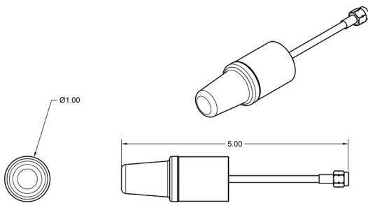
Technical Drawing
