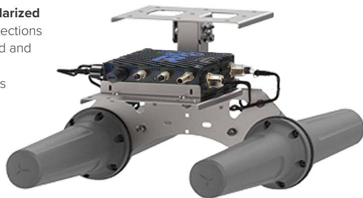
Rajant Hawk BreadCrumb and Poynting HELI-22 Dual Frequency Bi-Directional Mine and Tunnel Antenna System
