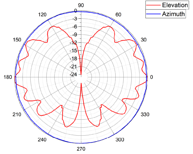
Radiation Patterns
