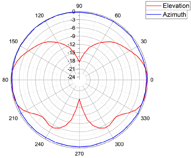
Radiation Patterns
